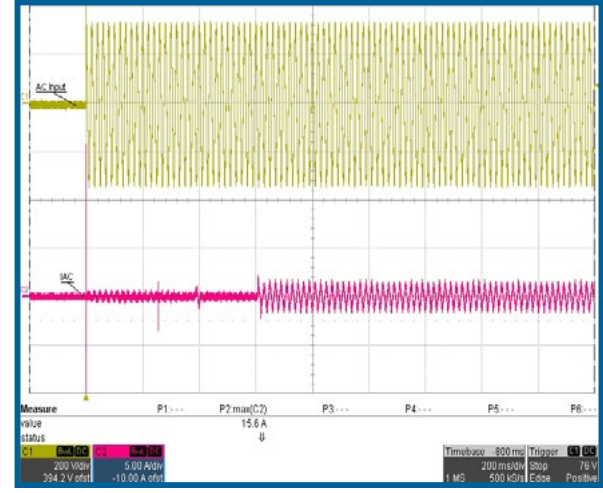
Inrush current at 230Vac - PST21D-28150
