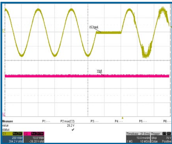
Input power brake at 230Vac 100% Load - PST21D-28150
